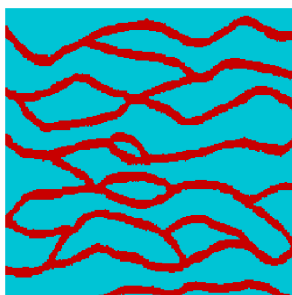
Strebelle' channels
